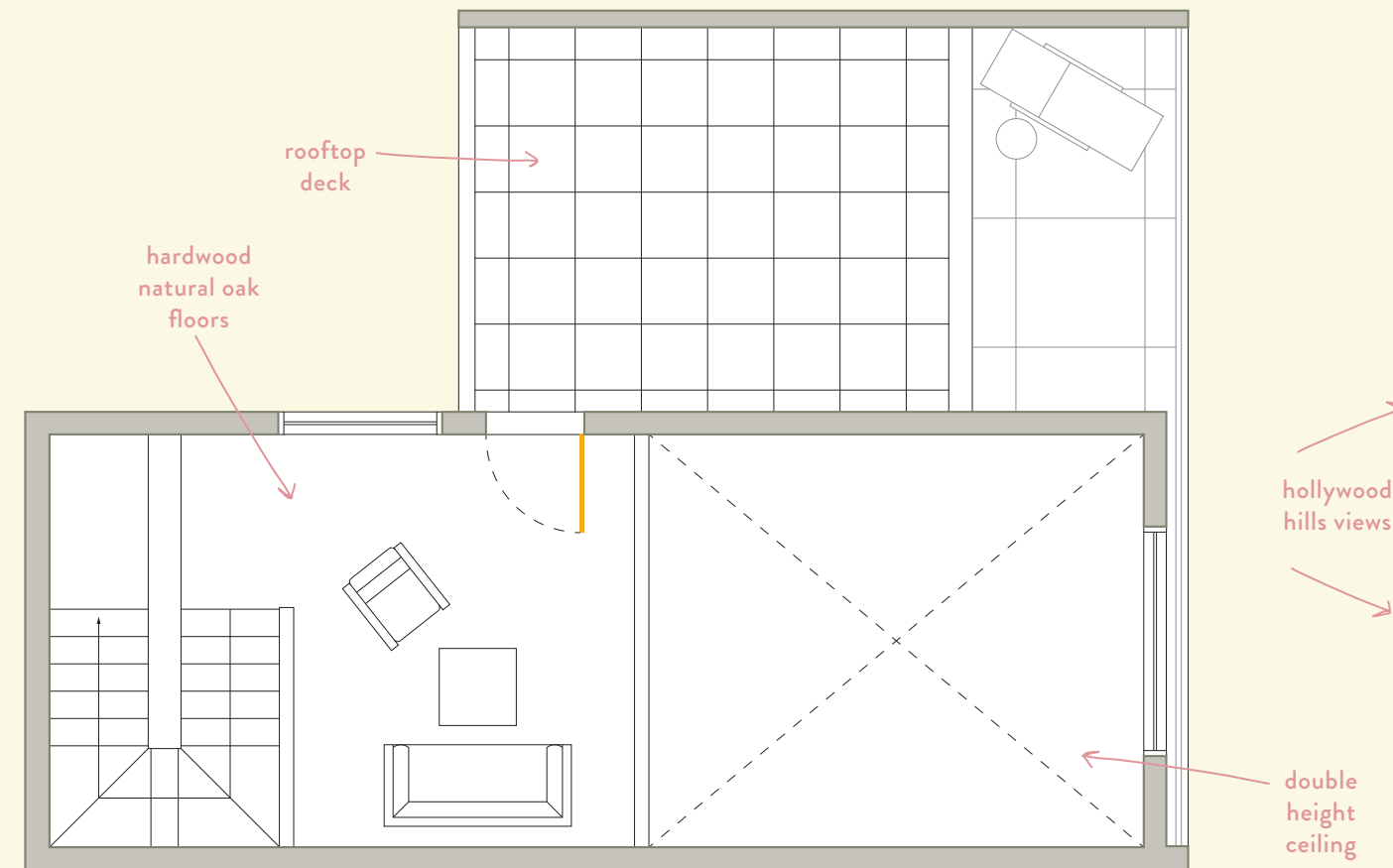
LEVEL 2
